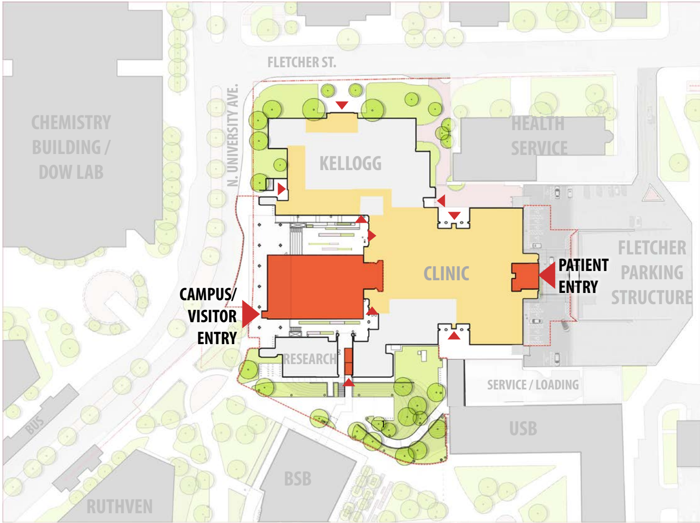
Site Plan
